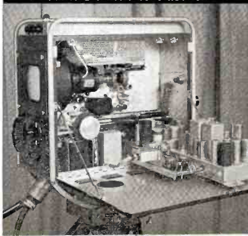
VERTICAL CHASSIS CONSTRUCTION
